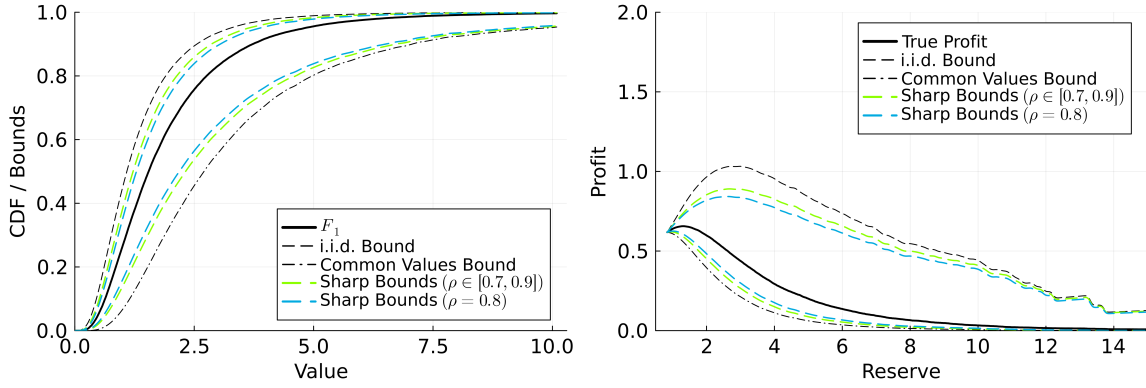
Figure 2: Simulated bounds on the CDF of the highest value and expected profit.
